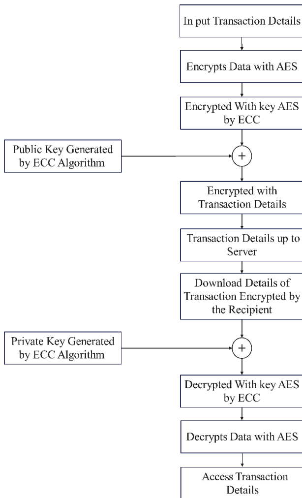
Figure 1. AES-ECC Encryption/Decryption
